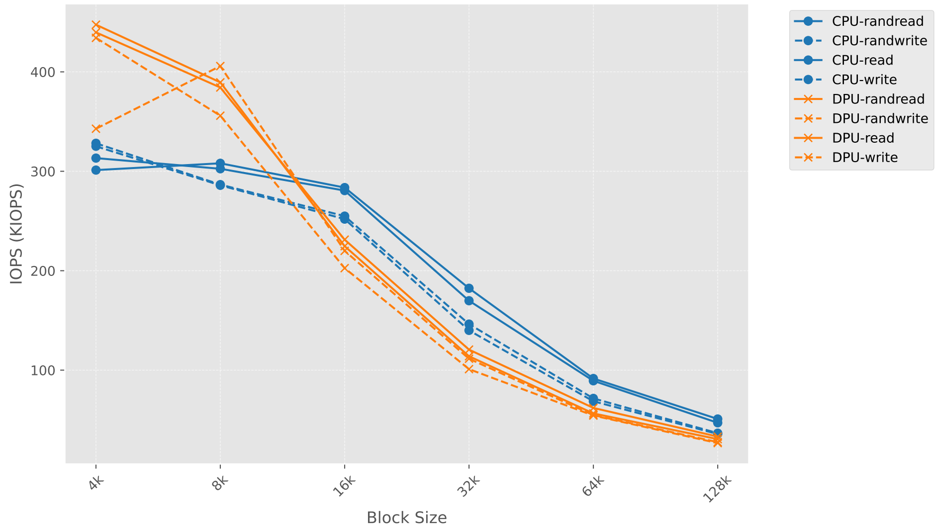
IOPS vs Block Size
